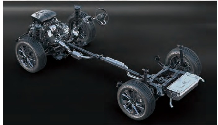
Front Macpherson Rear Multi-link Independent Suspension + 2WD
